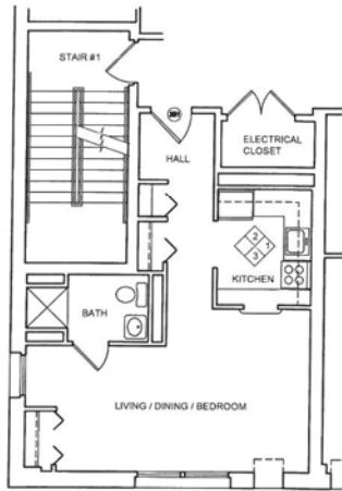
APT. TYPE B ENLARGED FLOOR PLAN SCALE: 1/4"=1'-0" AREA: 433 S.F. NORTH
