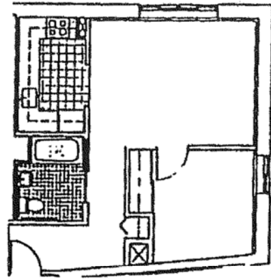
Apt. Style "B" Mobility Impaired Unit 525 sq. ft.
